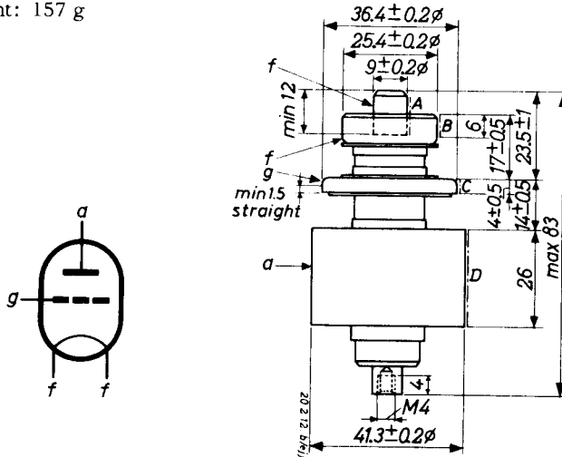
Fig. 1 Mechanical outline.
