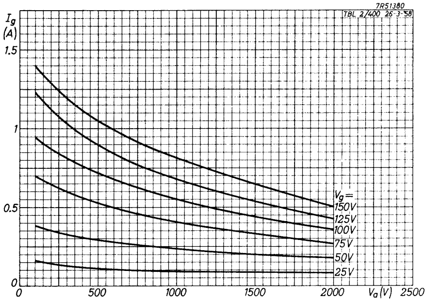
Fig. 3 I_g/V_a characteristics.
