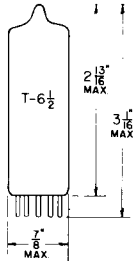
GLASS BULB
