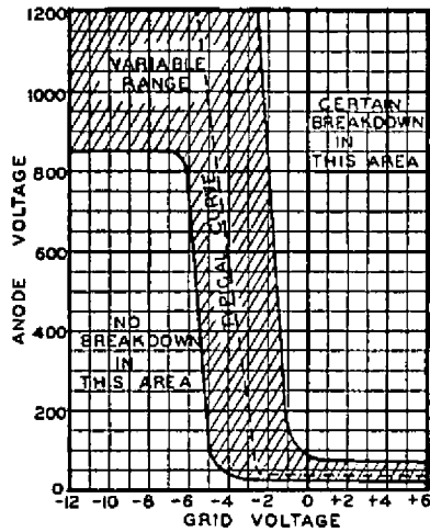
CONTROL CHARACTERISTICS
