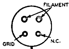
BOTTOM VIEW OF BASE
